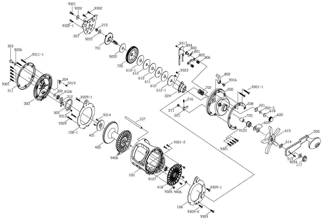
CV - 55S Spare Parts
